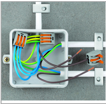
Wiring fine-stranded conductors in a junction box.
